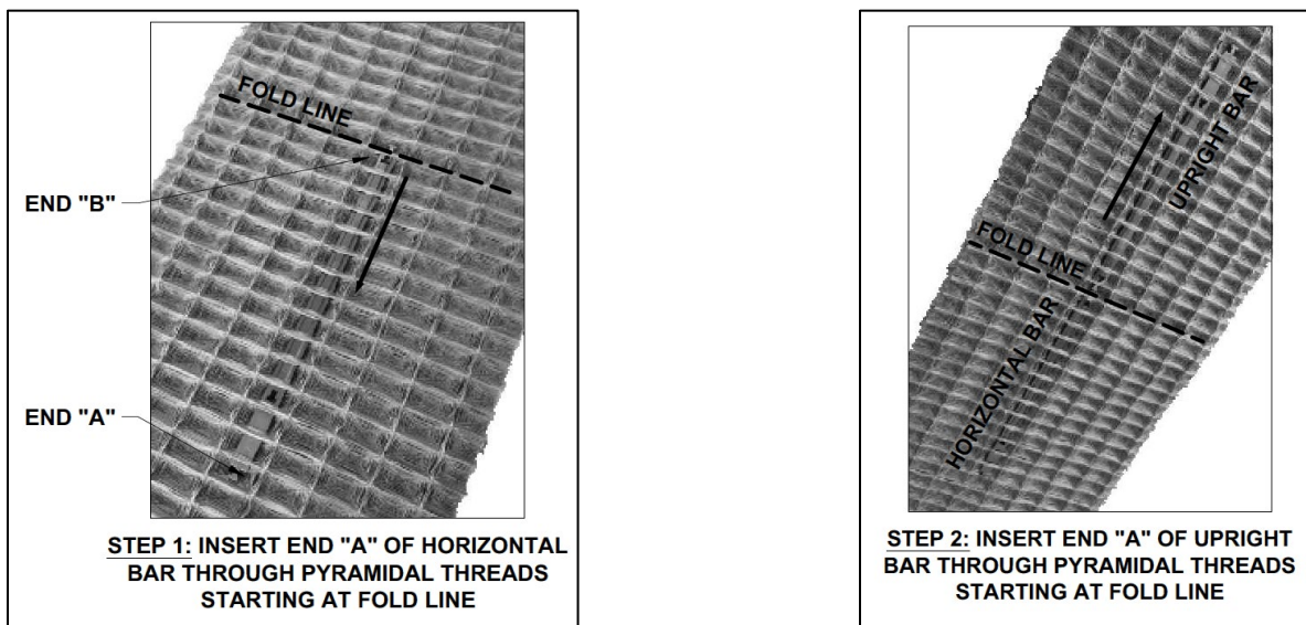
Figure 3 - Brace Component Assembly, Steps 1 and 2
