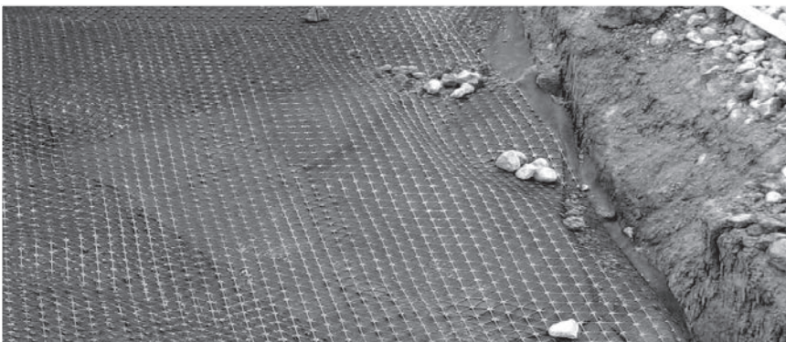
Anchoring geogrid with piles of aggregate.
